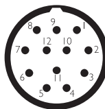
M23-Steckverbinder, 12-polig
